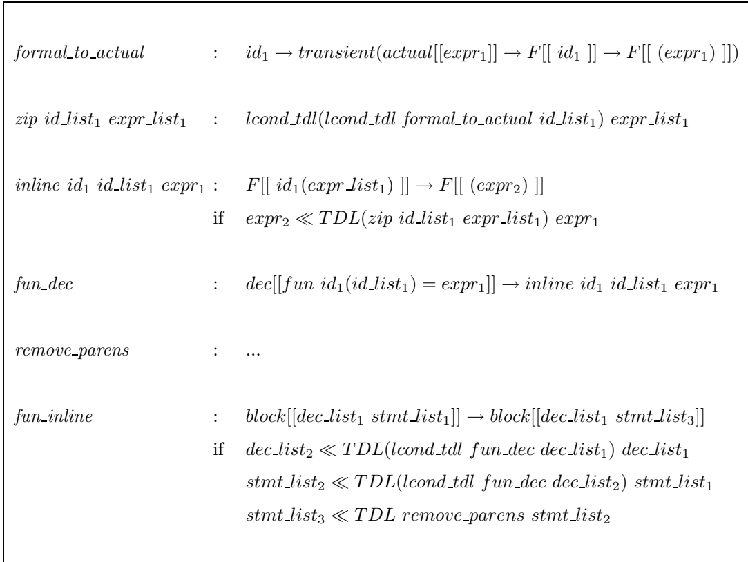
Fig. 18. A TL implementation of naïve function in-lining
