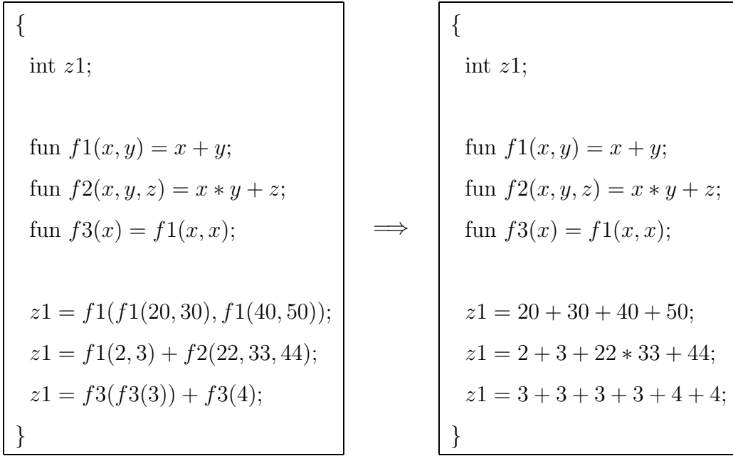
Fig. 17. An example of function in-lining
